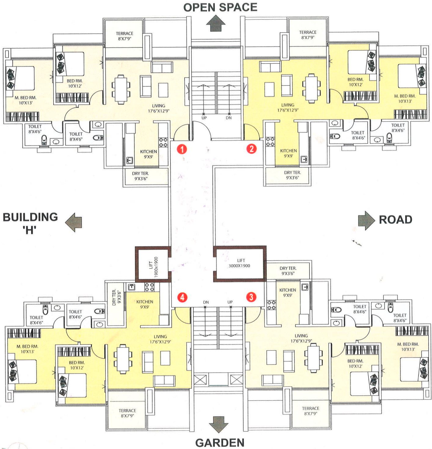
EVEN FLOOR PLAN
