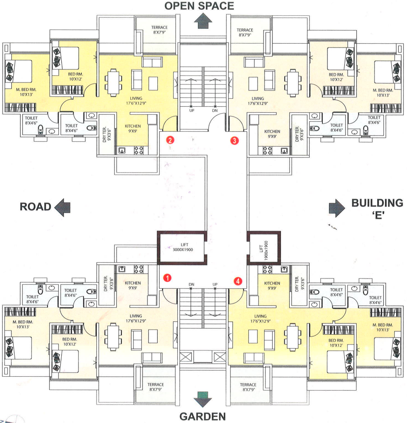
ODD FLOOR PLAN
